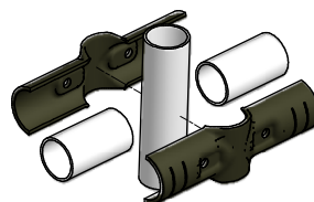
G4 CONNECTION
