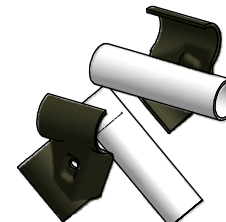
G10 CONNECTION
