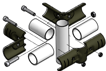
G3 CONNECTION
