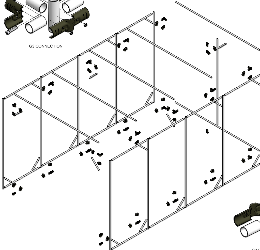
ASSEMBLY GUIDE
