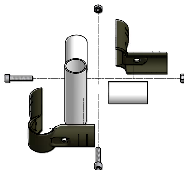
G2 CONNECTION
