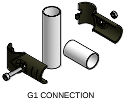
G1 CONNECTION
