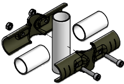
G4 CONNECTION
