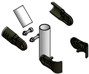
G7 CONNECTION
