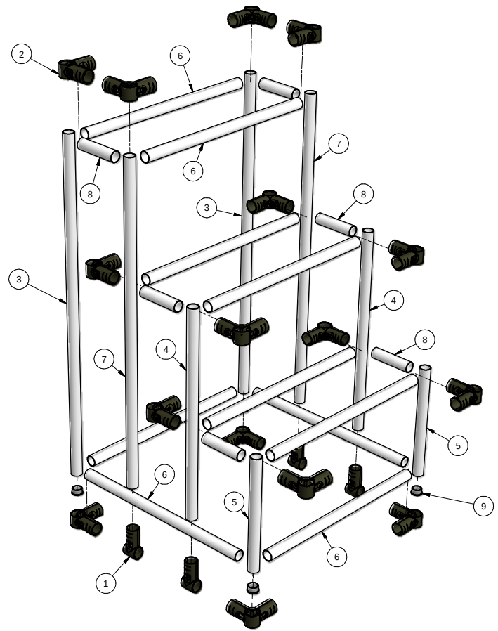
ASSEMBLY GUIDE
