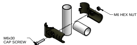
G1 CONNECTION
