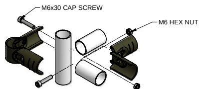
G2 CONNECTION
