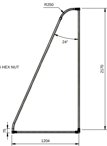
END VIEW
