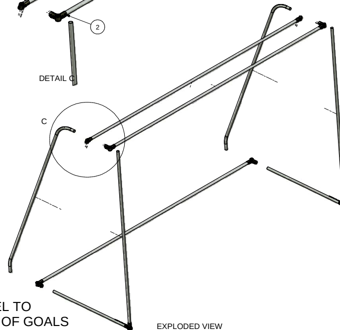
EXPLODED VIEW
