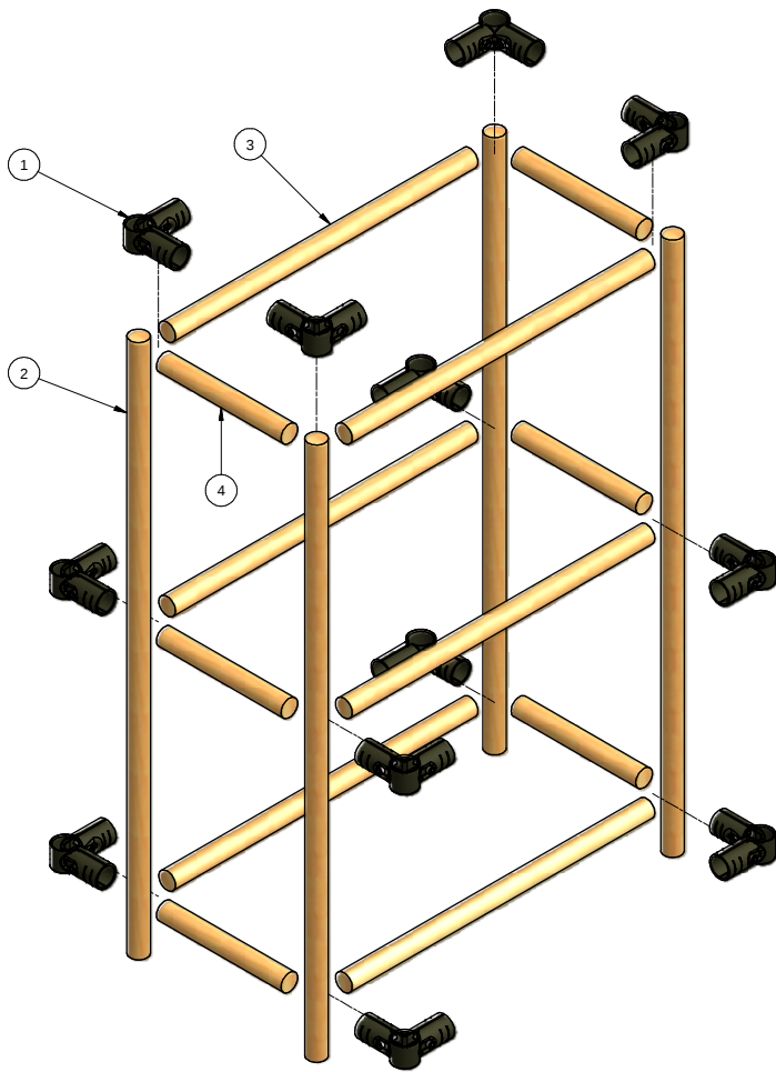
ASSEMBLY GUIDE
